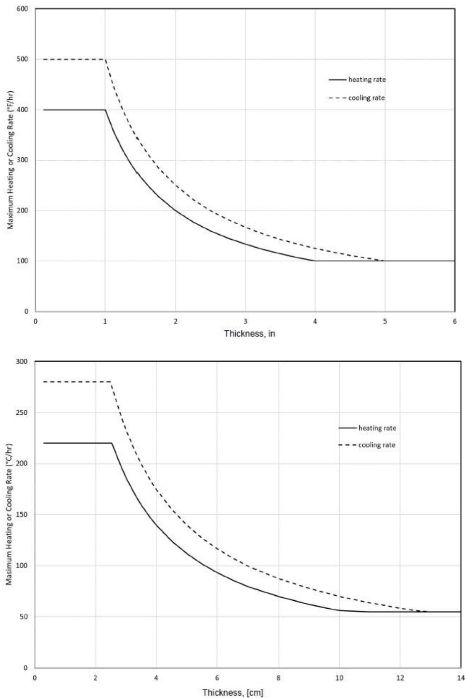
Figure C-7.9—Maximum Heating and Cooling Rates
